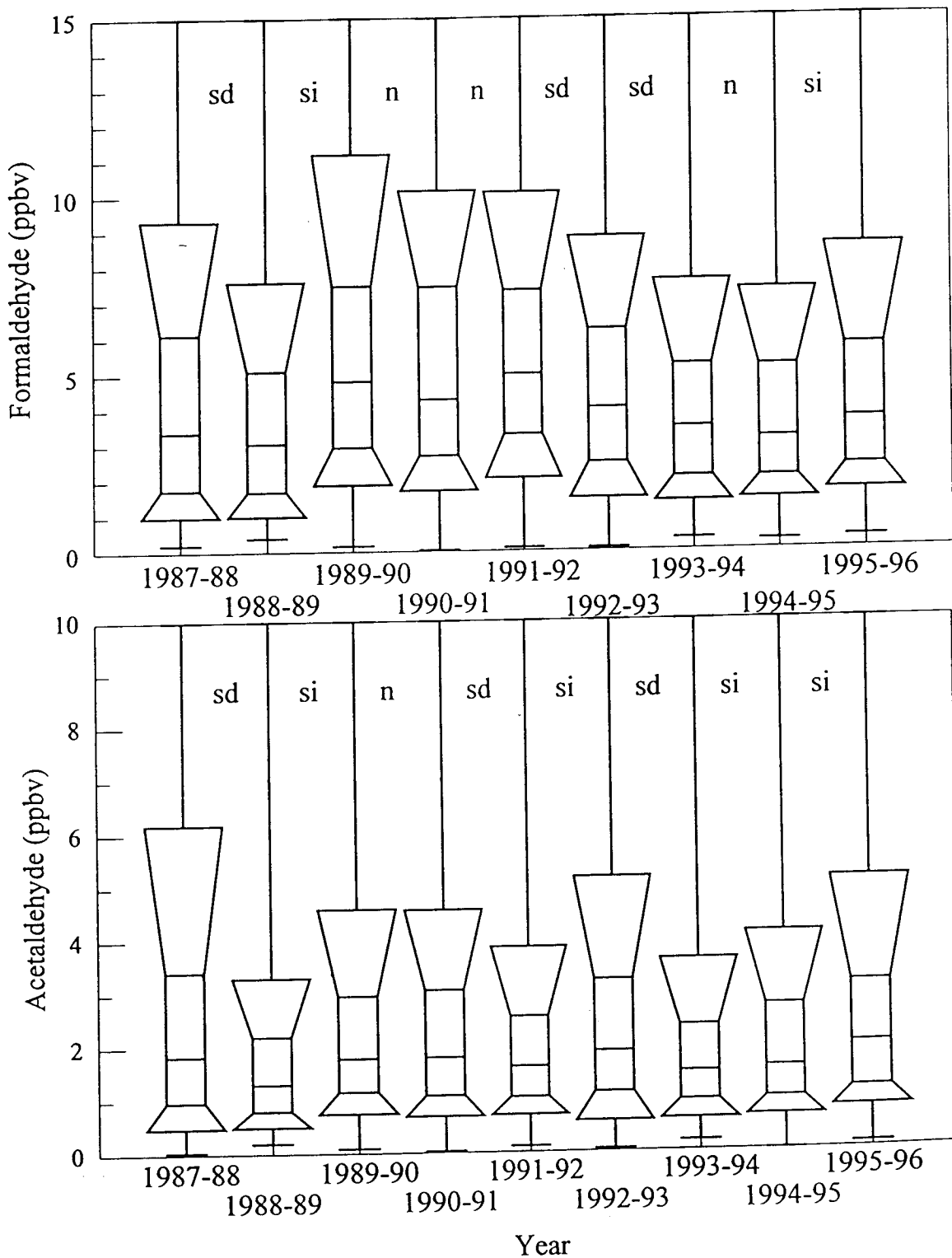
Figure 1. Box plots of the winter average formaldehyde and acetaldehyde concentrations measured in downtown Denver for the winters of 1987-88 through 1995-96. The horizontal lines in the box plot have the following meanings, proceeding from the bottom to top: the line at the bottom represents the lowest concentration measured, the line forming the bottom of the box is the 10th percentile, next is the 25th percentile; near the middle of the box is the median, then the 75th percentile, and 90th percentile. The maximum concentration measured is off scale of the plots.
