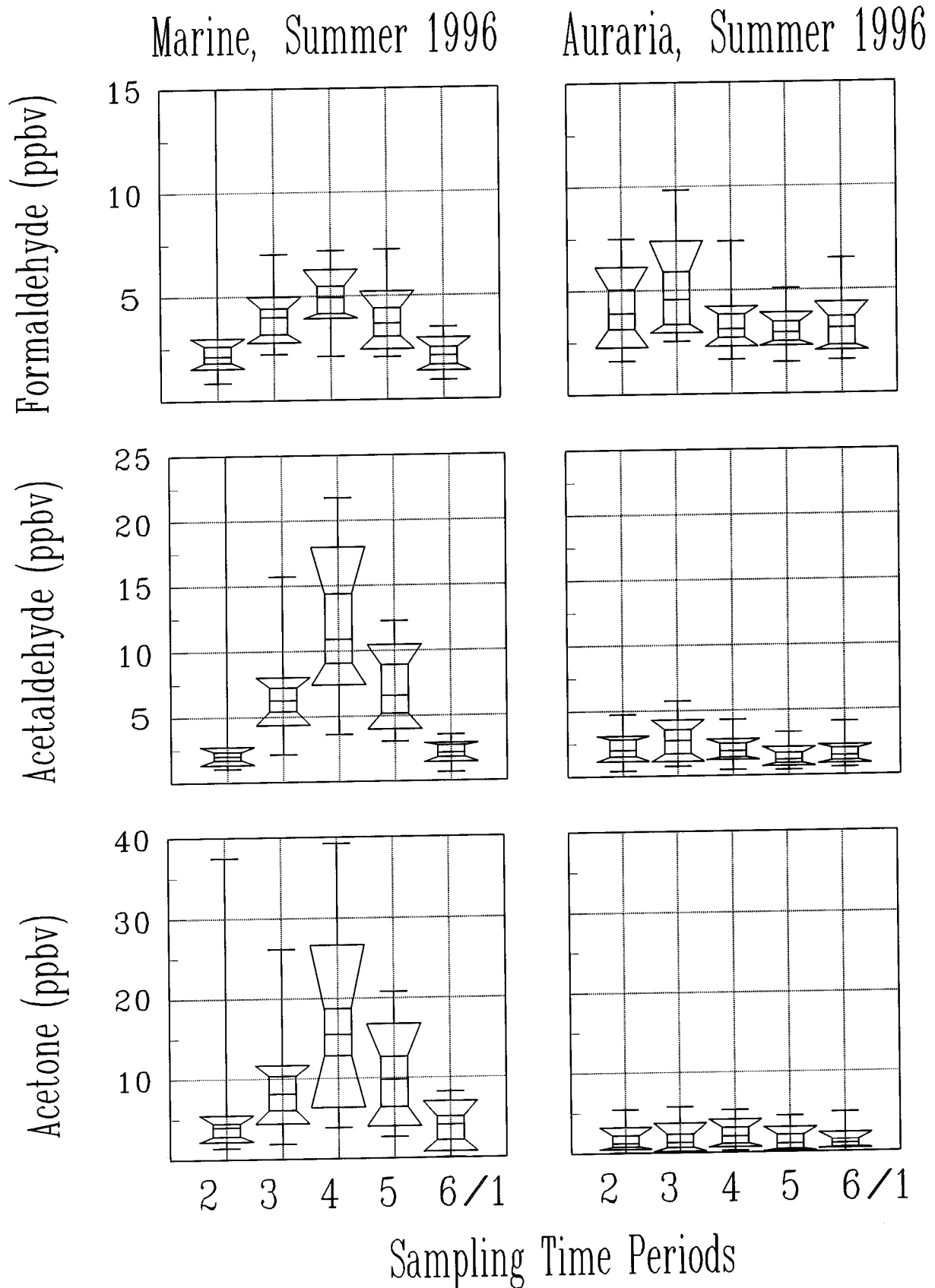
Figure 4. Box plots of the diurnal character of formaldehyde, acetaldehyde, and acetone (all in ppbv) at Marine, and Auraria for the summer (July 12 - Sept 1) 1996 sampling period. Note the differences in the scales for the y axes. See Results (summer 96) section of text for explanation of box plots.
